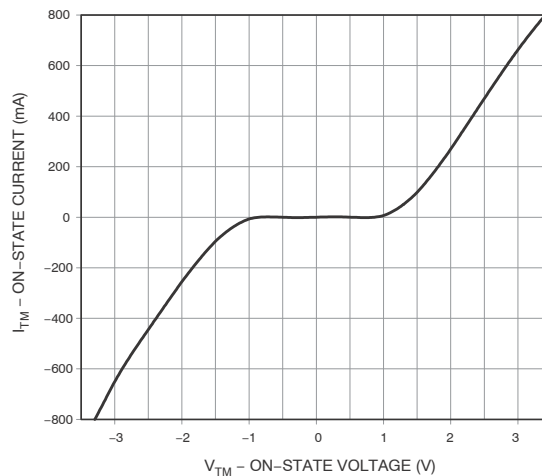
Figure 3. On-State Characteristics
