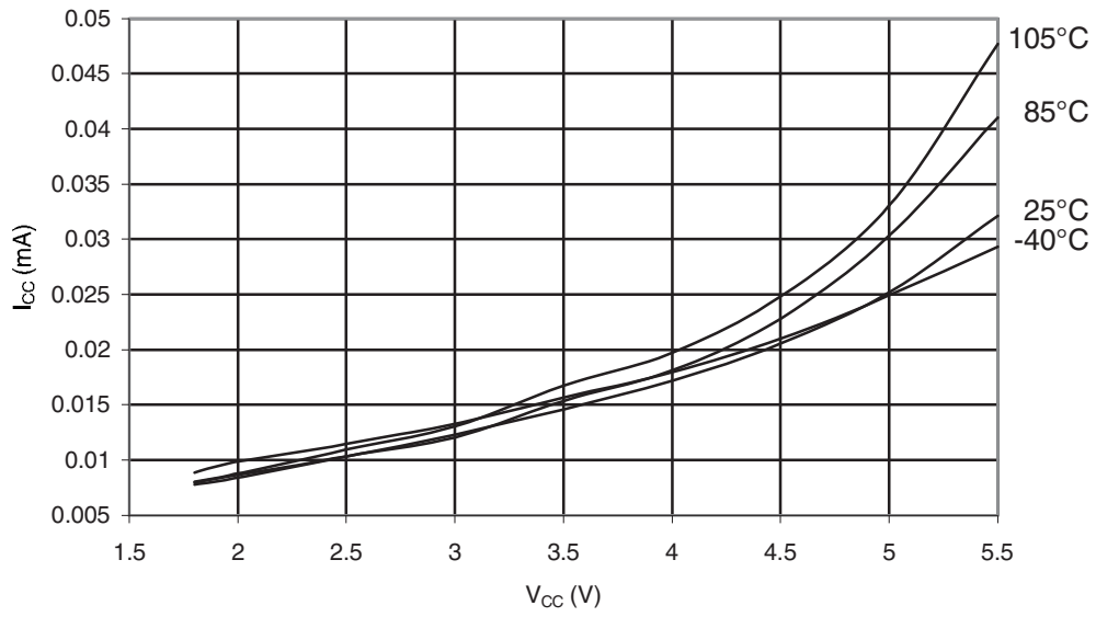
Figure 35-8. ATmega328P: Idle Supply Current vs. V_{CC} (Internal RC Oscillator, 128kHz)
