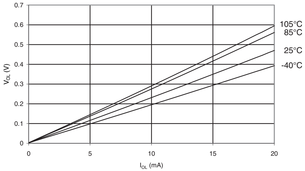
Figure 31-353. ATmega328P: I/O Pin Output Voltage vs. Sink Current ( V_{CC} = 5V )
