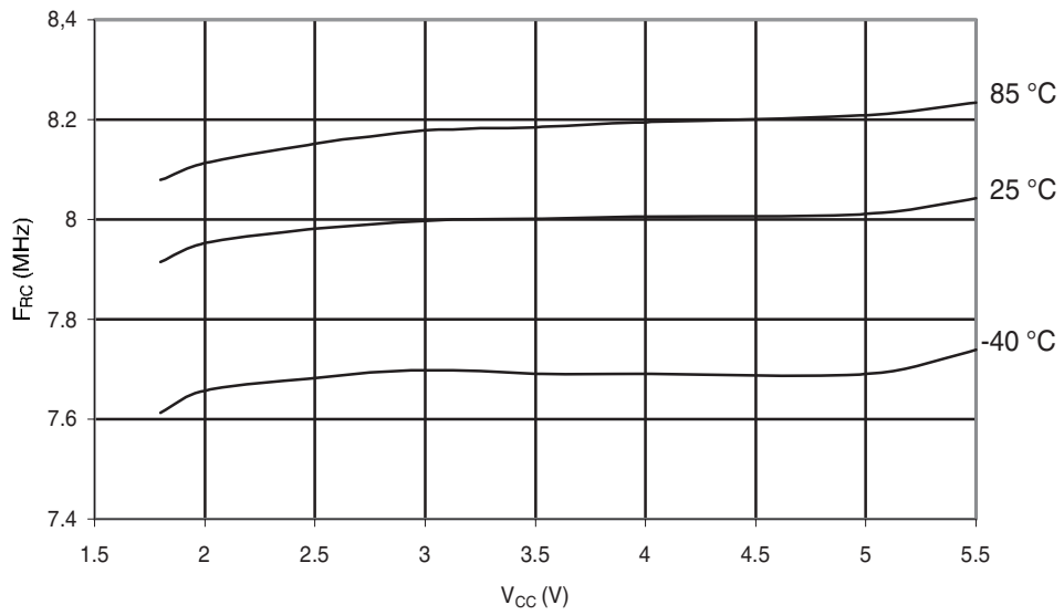
Figure 31-226. ATmega168A: Calibrated 8MHz RC Oscillator Frequency vs. V_{CC}
