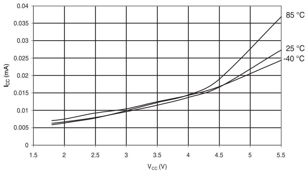
Figure 31-197. IATmega168A: Idle Supply Current vs. V_{CC} (Internal RC Oscillator, 128kHz)
