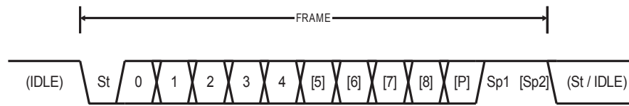
Figure 20-4. Frame Formats
