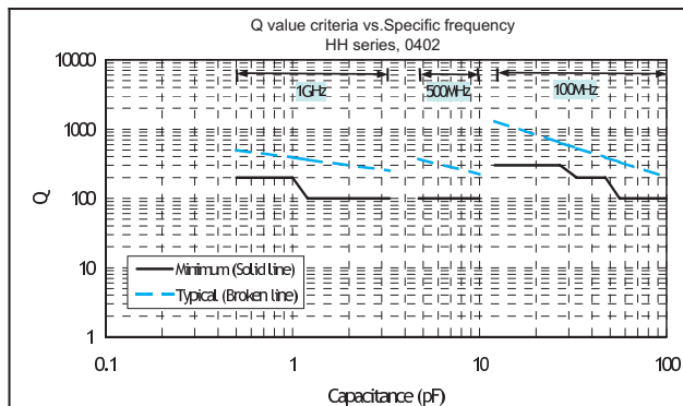
Fig. 1 Q factor specification vs. Specific frequency 0402
