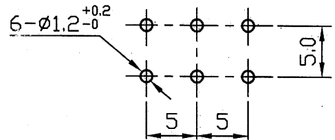
MOUNTING HOLE DETAIL
